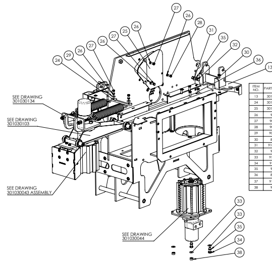
CHIPPER CHAMBER ROLER BOX 301020101 ARB190 ROLLERS
