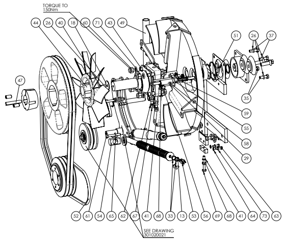
301020113 FLYWHEEL DRIVE DETAIL ARB190
