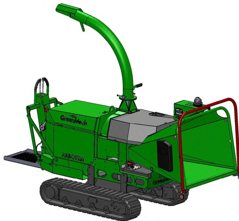
ARBTRAK DIESEL ENGINE 34HP TD KUBOTA
