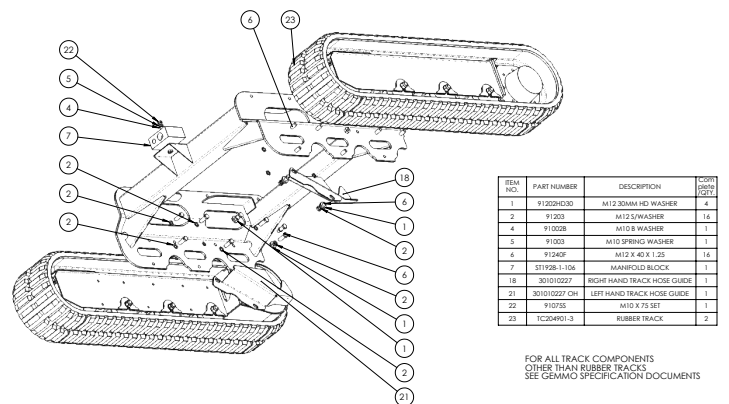
TRACKED CHASSIS SUBFRAME 301010275 ARB190 & 200
