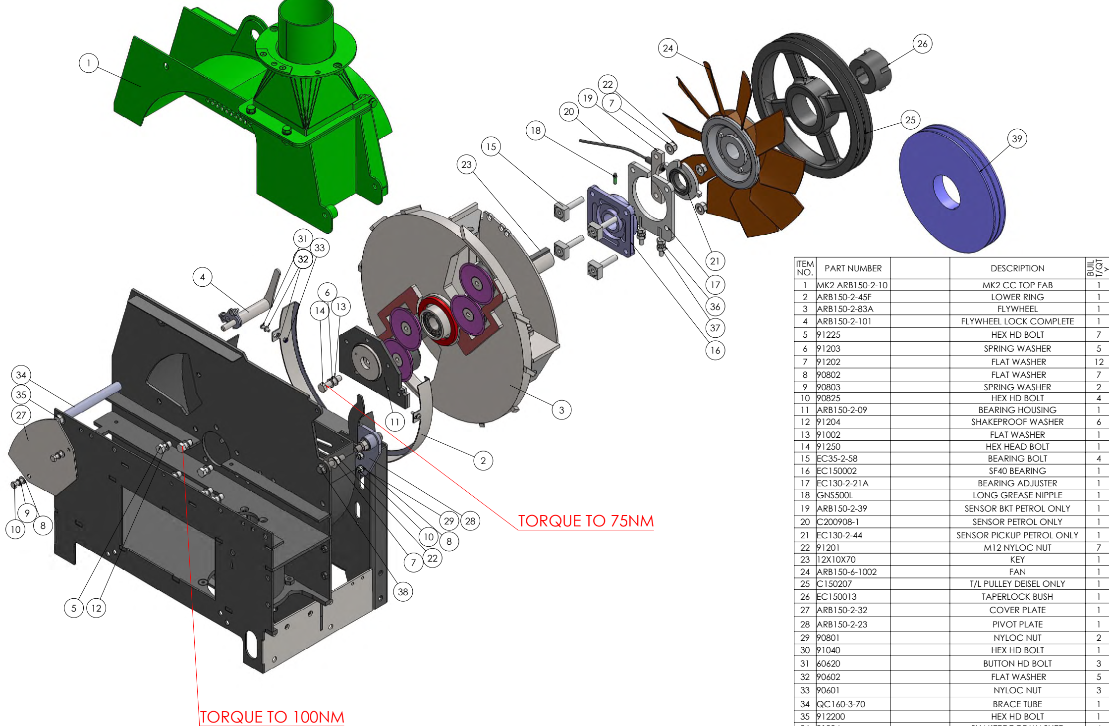
ARB150-2-ARB150-3MK2 FLYWHEEL
