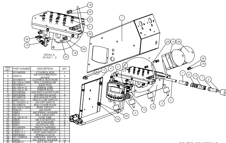
CONTROL BOX TOP BAR 301040025 ARB190
