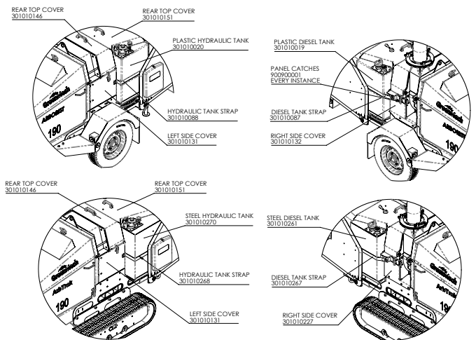
ARB 190 COVERS
