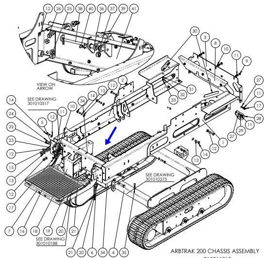
ARBTRAK 200 CHASSIS ASSEMBLY 315011010
