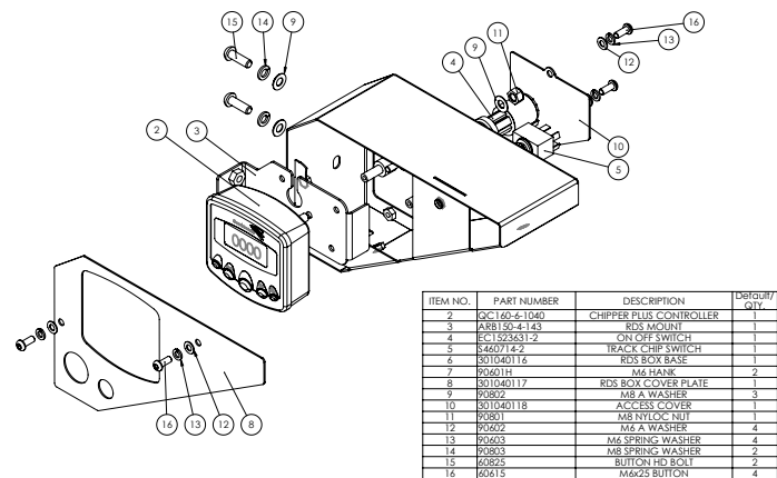
RDS SURROUND BOX 301040114 ARB190 & 200
