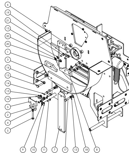
315021000 CHIPPER CHAMBER & ROLLBOX SHEARBARS VIEW
