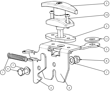
BONNET LATCH ASSEMBLY 301010093 ARB190 & 200
