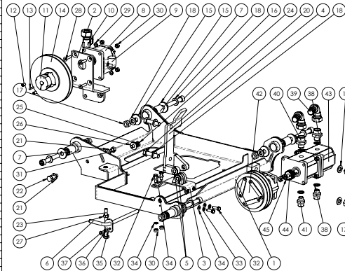
ARBTRAK 200 ENGINE TRAY 315060020
