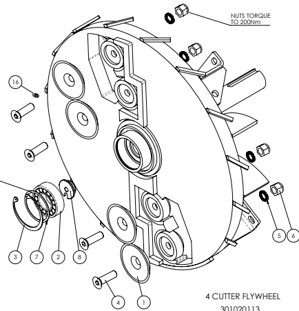
4 CUTTER FLYWHEEL 301020113 ARB190 & 200
