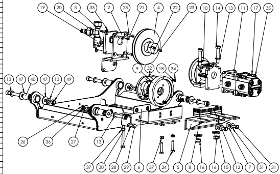
ARBTRAK 190 ENGINE TRAY 301060073
