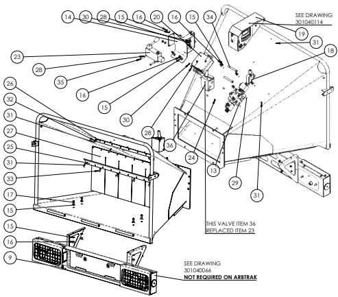
INFEED CHUTE 301040050 ARB19 NEW INFEED & FLAP
