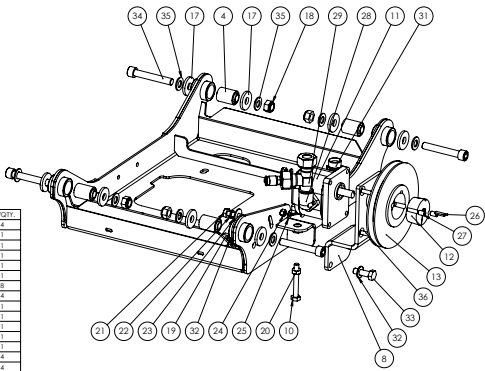
ENGINE TRAY 301060016 ARBORIST 190 & 200
