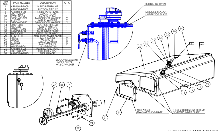
PLASTIC DIESEL TANK ASSEMBLY 301010019 ARB190/200 REV 1A NEW INPBD & FLAP
