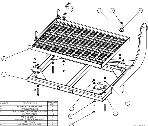
PLATFORM BASE 301010188 ARBTRAK 190 & 200
