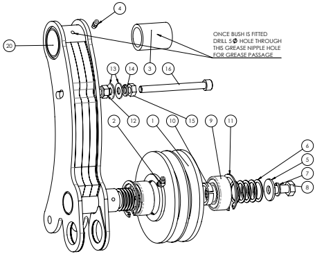
BELT TENSIONER BRACKET 315021034 ARB200
