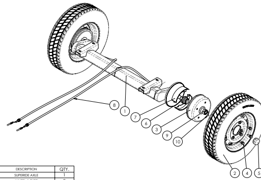
SUPER RIDE AXLE ARB190-9-1018
