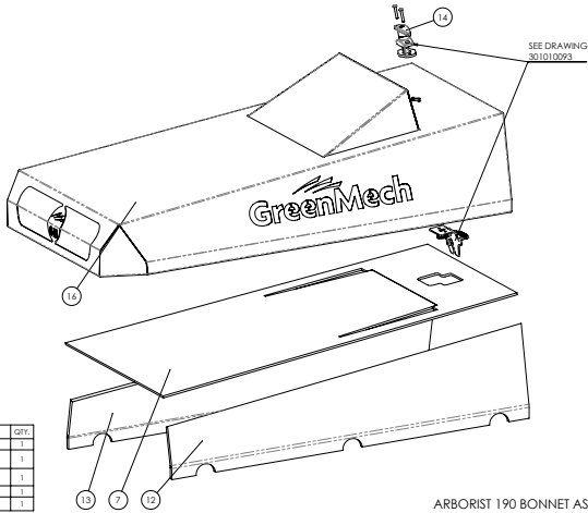
ARBORIST 190 BONNET ASSEMBLY 301010332
