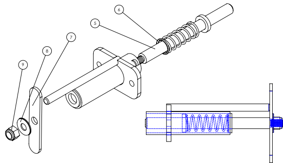
FLYWHEEL SPRING BOLT LOCK 301020065
