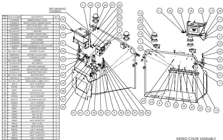
INFED CHUTE ASSEMBLY 315040054 ARB200
