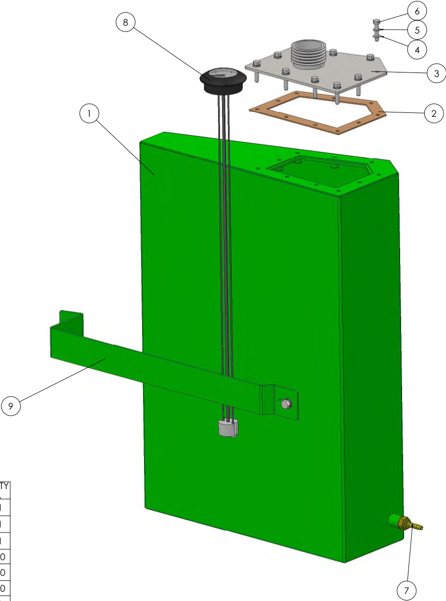
STEEL TANK FOR PETROL MACHINES
