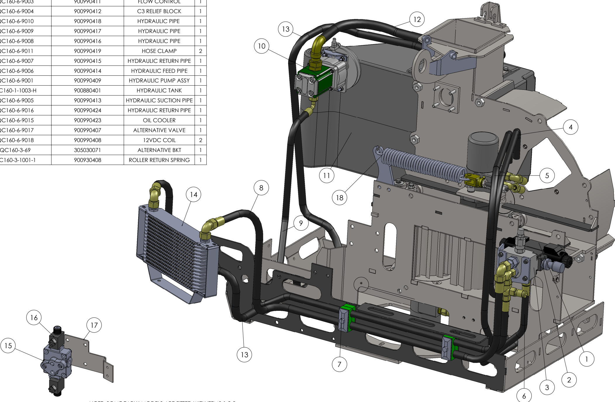
HYDRAULIC LAYOUT WITH OIL COOLER
