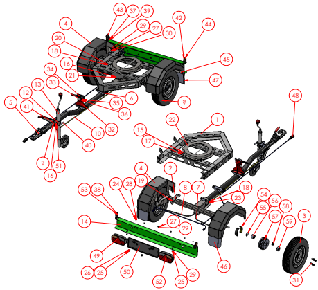
MK2 AXLE-CHASSIS FRAME
