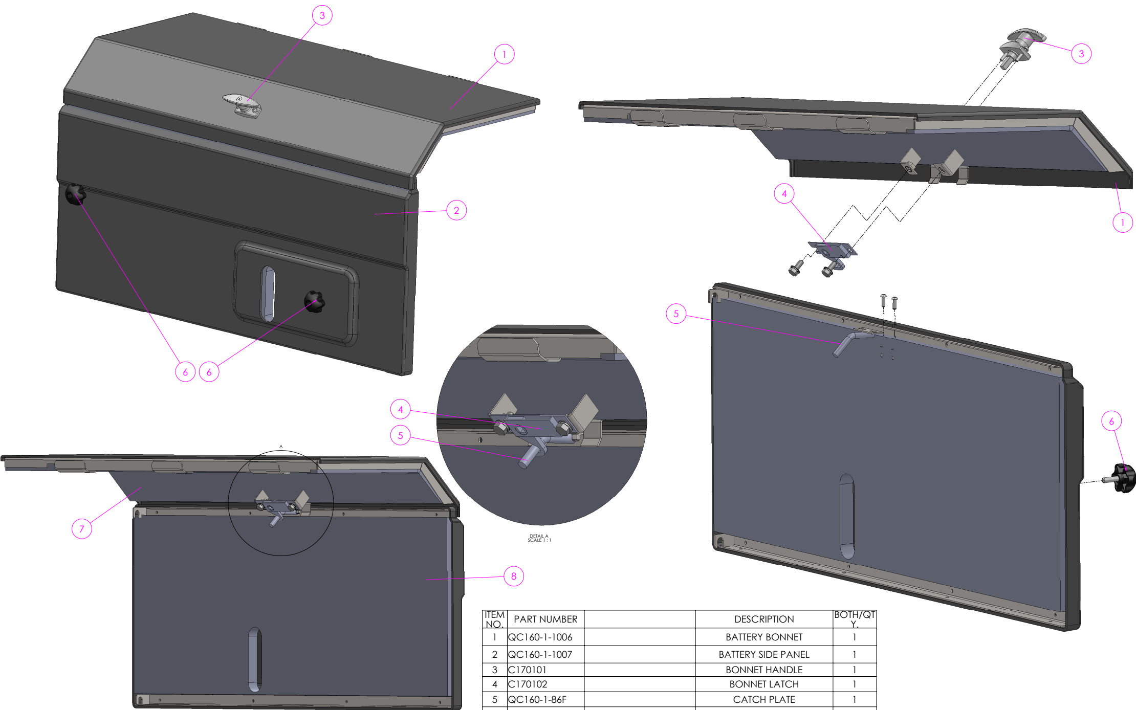
BATTERY BONNET & SIDE PANEL
